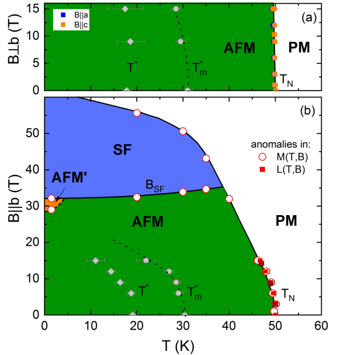
FIG. 6. Magnetic phase diagram of LiFePO 4 for (a) B||a (blue markers), B||c (orange) and (b) B||b (red) as constructed from thermal-expansion/magnetostriction (squares) and magnetization (circles) measurements. The lines are guides to the eye. AFM, AFM', SF, and PM label antiferromagnetically ordered, spin-reoriented, and paramagnetic phases, respectively. T_N , B_{C1} , and B_{SF} label the associated anomaly temperatures and fields. T^* ( T_m^* ) labels the inflection point (minimum) associated with the low-temperature features in \alpha_b and \alpha_c (grey markers; see the text).
