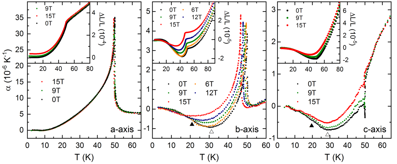
FIG. 3. Thermal-expansion coefficient \alpha at magnetic fields between 0 and 15 T for all three crystallographic directions of \text{LiFePO}_4 . Insets show the corresponding length change. Open (filled) triangles label the temperatures T_m^* ( T^* ) of a minimum (inflection point) in \alpha (see the text).
