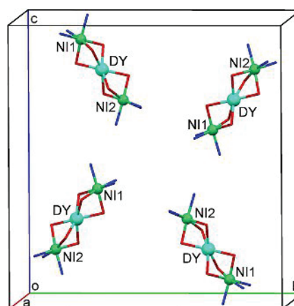
Figure 2. Orientation of the molecules in the unit cell of [Dy^{III}\{Ni^{II}(L)\}_2]ClO_4 .
