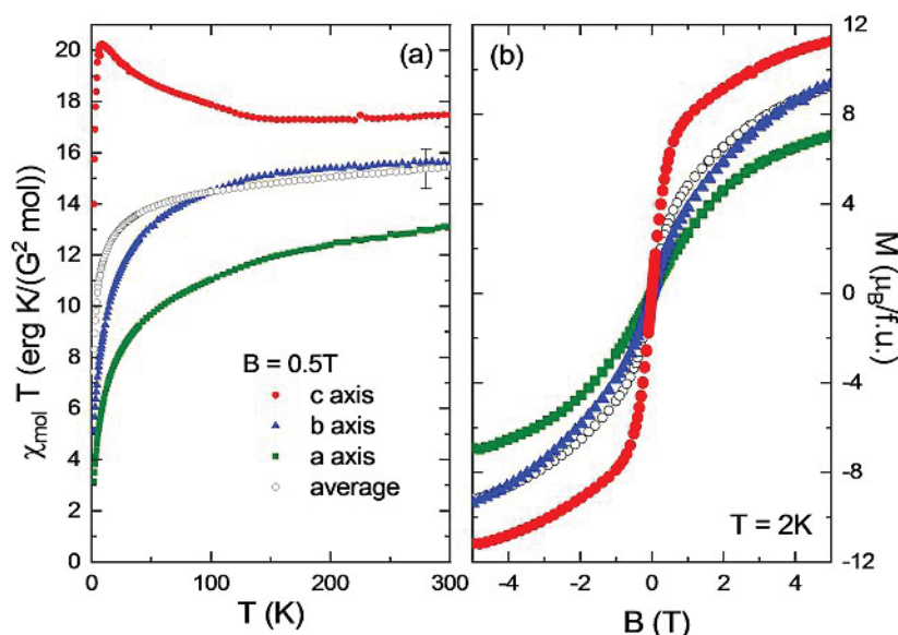
Figure 3. a) Temperature dependence of \chi_{\text{mol}} T vs. T along the three crystallographic axes at B = 0.5 T (colored) and its average (black). (b) Field dependence of the magnetization along the three crystal axes and its average, at T = 2 K.
