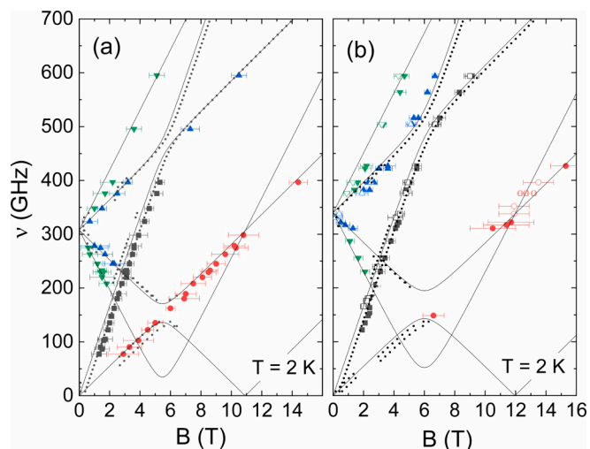
Fig. 9. Frequency vs. magnetic field diagram of complexes 1 (a) and 2 (b). The dotted lines show simulations using the SH in Eqn. (1) extended by finite exchange coupling (see the text) between two neighbouring spins. D and E anisotropy parameters as well as g_z -values equal those of the single-ion model represented by the solid lines (cf. Table 1). The open symbols in panel (b) represent the resonance branches observed in a magnetically diluted sample of 2.
