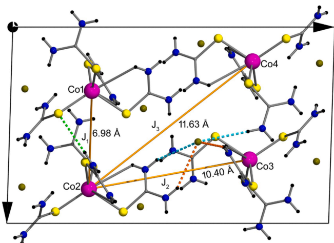
Fig. 2. The packing diagram of 1 (view along the b -axis) shows the interatomic distance between the molecules in the crystal lattice. The dotted bonds represent the intermolecular H-bonding between the molecules in the crystal lattice.
