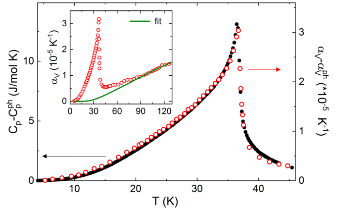
FIG. 4. Grüneisen scaling of the magnetic contributions to the heat capacity c_p^{\text{mag}} and volume thermal expansion coefficient \alpha_v^{\text{mag}} . Inset: The volume thermal expansion coefficient \alpha_v along with a combined Debye-Einstein fit to the high-temperature data (see the text).
