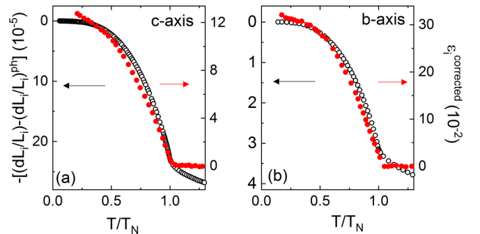
FIG. 8. Scalings of the nonphononic relative length changes dL_i/L_i and corrected dielectric permittivity \epsilon digitized from Dubrovina et al. [21] for the (a) c and (b) b axes respectively.
